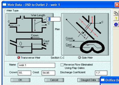
Weir
